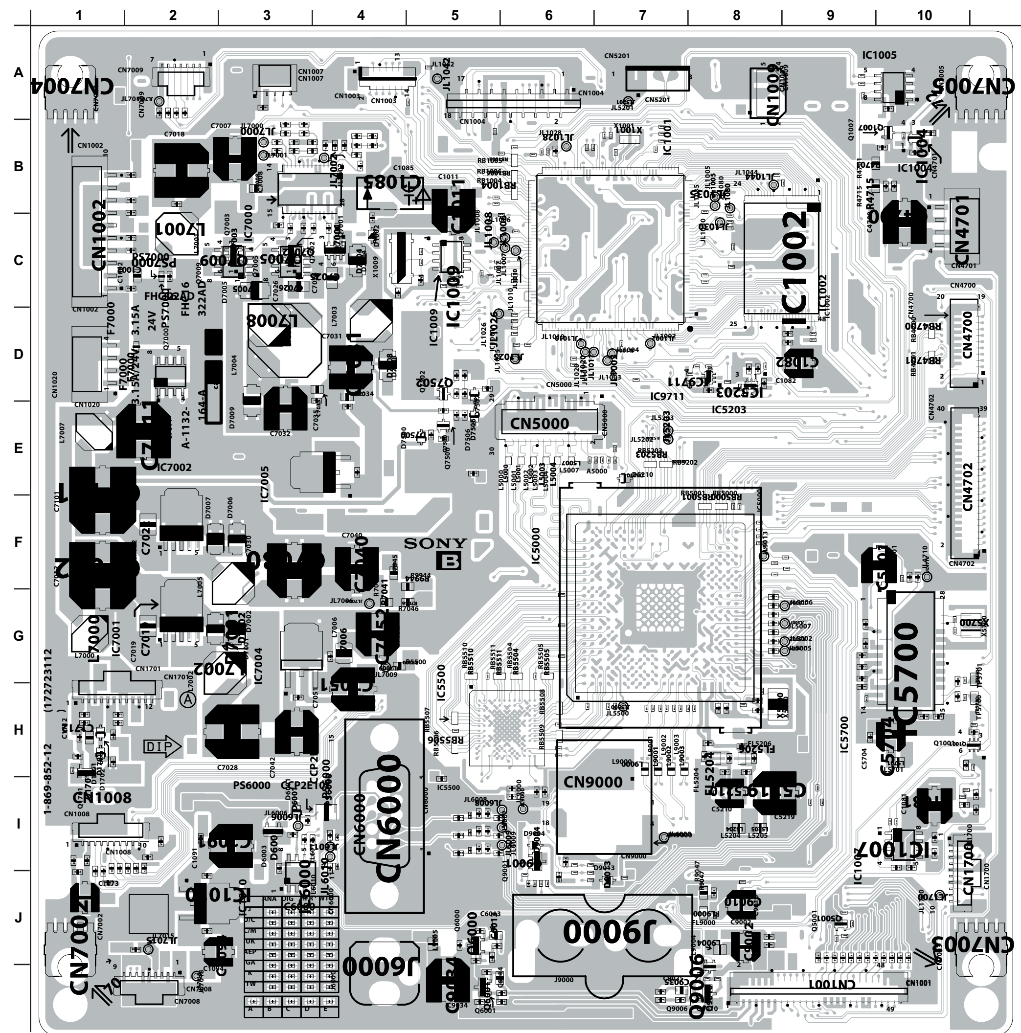
BU [MICRO, VIDEO PROCESSOR, SVP-PX(2/2) DDR & CPU I/F, POWER & GND VIDEO PROCESSOR, DPR_SDRAM 128MBIT, PC IN, HDMI, PANEL5V & FE5V, POWER SUPPLY] COMPONENT SIDE
