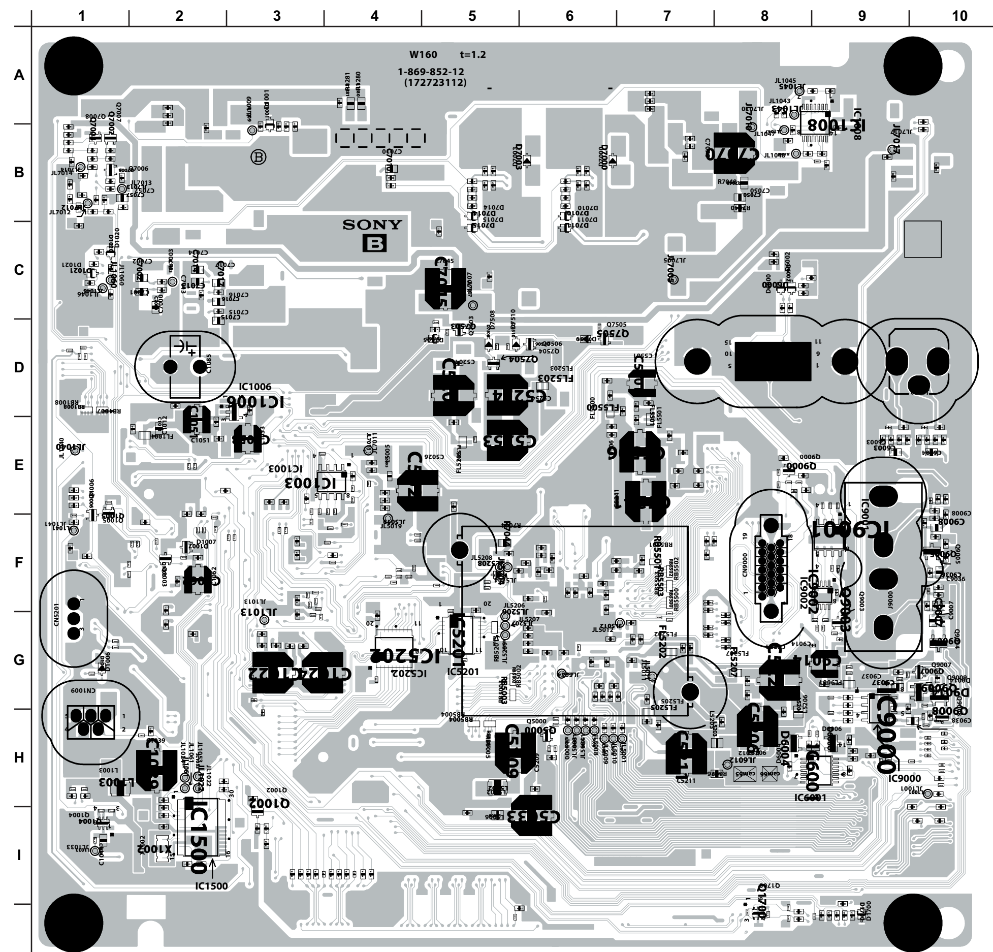
BU [MICRO, VIDEO PROCESSOR, SVP-PX(2/2) DDR & CPU I/F, POWER & GND VIDEO PROCESSOR, DPR_SDRAM 128MBIT, PC IN, HDMI, PANEL5V & FE5V, POWER SUPPLY] CONDUCTOR SIDE
